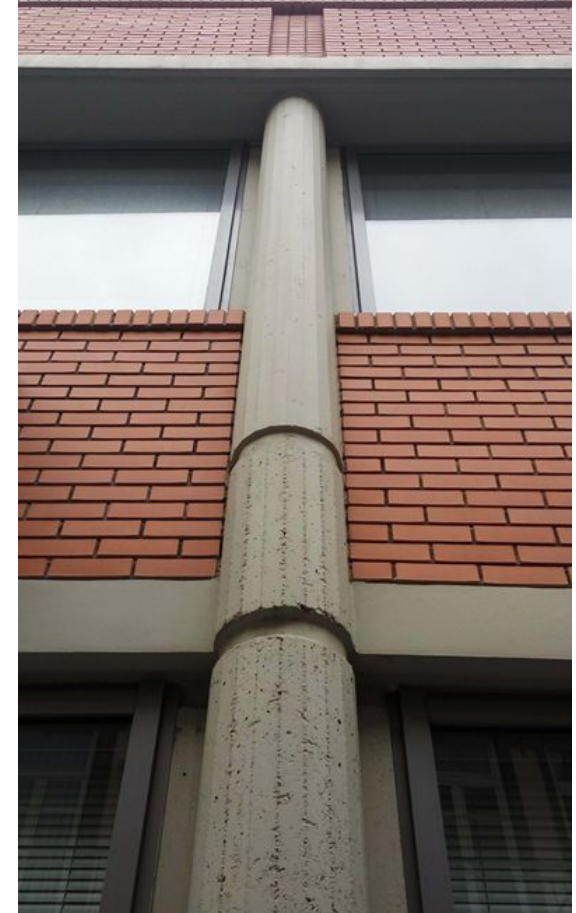
formworks cutted by laser-cutter, custom-made for the construction of the reinforced concrete columns
